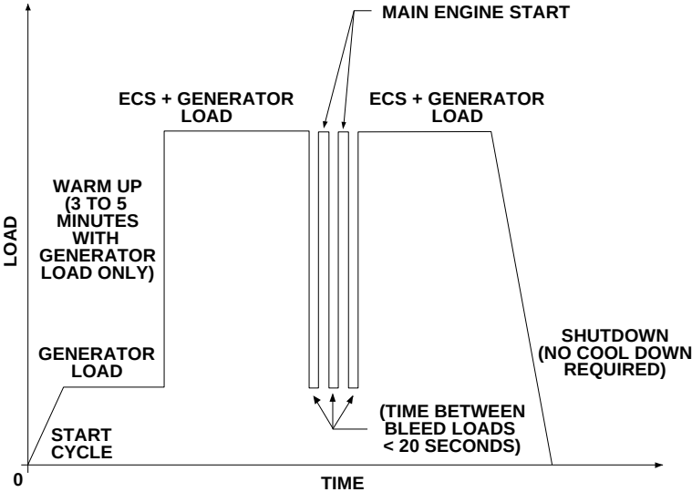
APU Cycle Profile For Optimum Turbine Wheel Life
