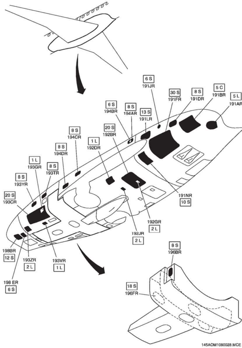
FIGURE 5 - EMB-145XR
