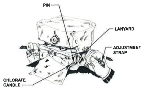
Figure 6 Lanyard Attachment
