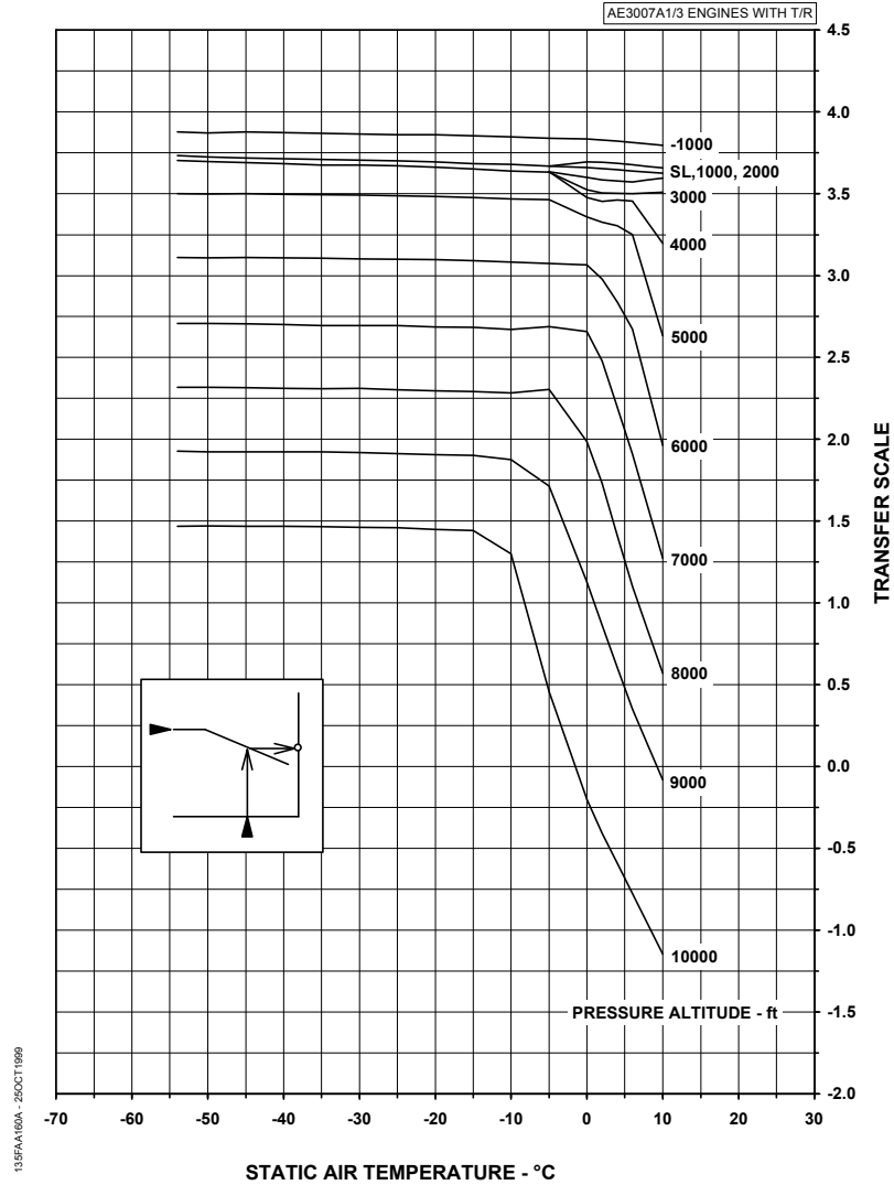
OBSTACLE CLEARANCE - REFERENCE GRADIENT (STANDARD CG) ALT T/O MODE - FLAPS 18° - BLEED OPEN - PACKS OFF - FADEC REF A/ICE ON CHART 1 OF 2
